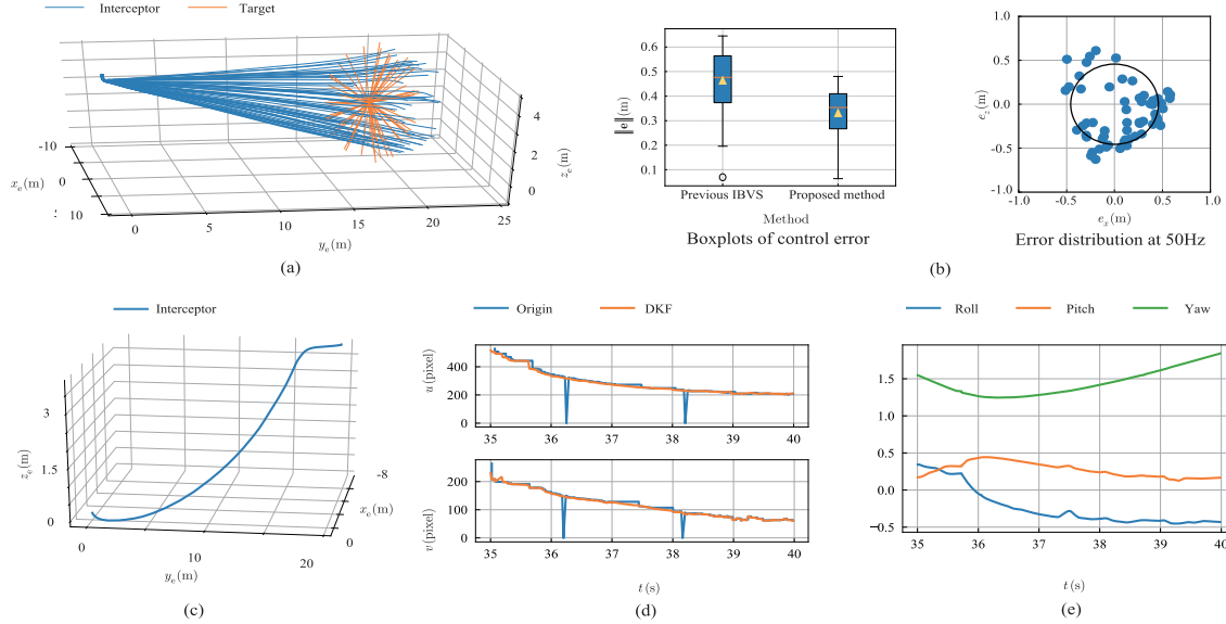
Fig. 10. Statistical results and single intercept details for comparison with previous IBVS methods. (a) Trajectories in statistics. (b) Error distribution of the previous IBVS and the proposed method. (c) Trajectory of a single interception. (d) Image coordinates. (e) Interceptor attitude.
